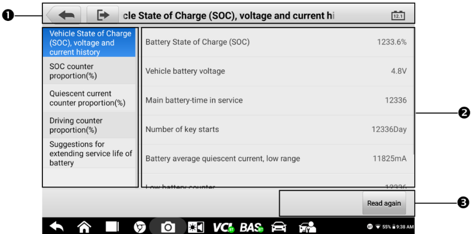
Figure 7-5 Sample Battery Usage History Screen
