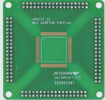
APB107 (MCU_FQFP144) * 1
