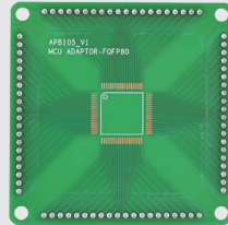
APB105 (MCU_FQFP80)
