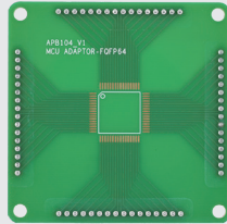
APB104 (MCU_FQFP64) * 1
